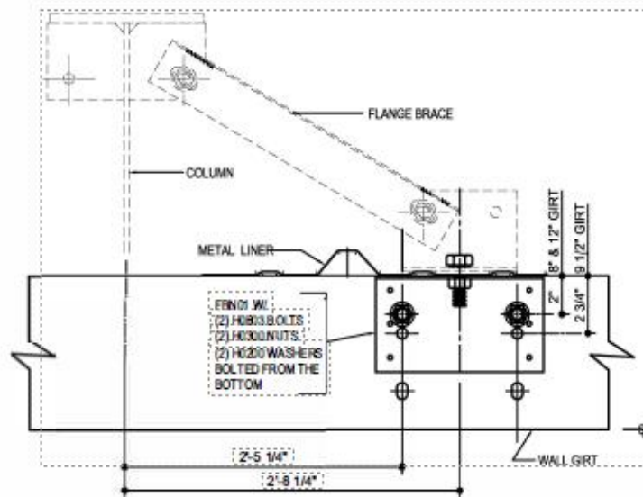
TYPICAL FLANGE BRACE @ GIRT & COLUMN W/ LINER
