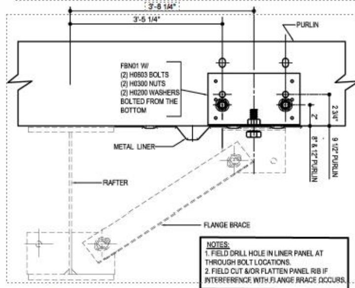
TYPICAL FLANGE BRACE @ PURLIN & RAFTER W/ LINER
